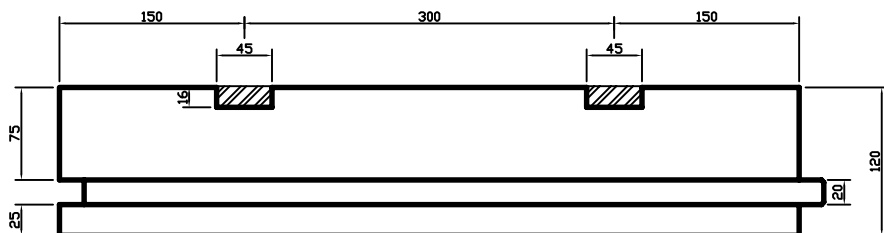
IsoCrafts U120
